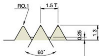
排齒詳圖 Drawing of Serration
