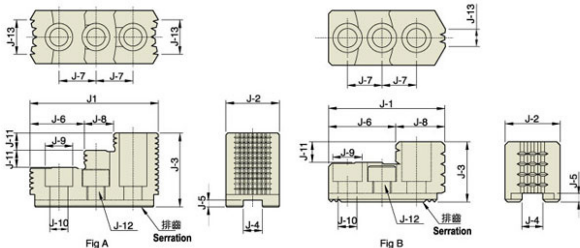
排齒詳圖 Drawing of Serration
