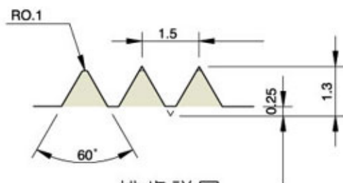
排齒詳圖 Drawing of Serration
