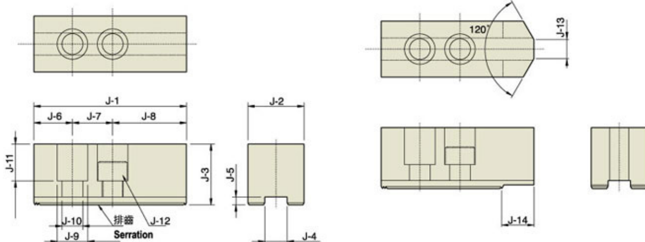
排齒詳圖 Drawing of Serration
